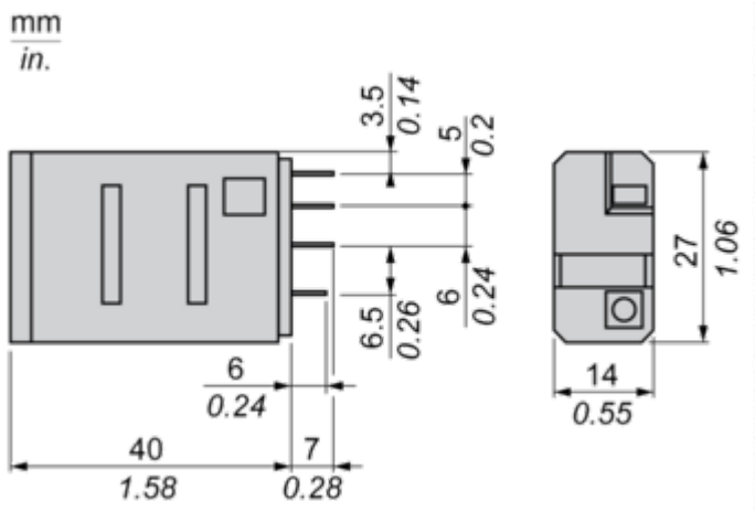
Pin Side View
